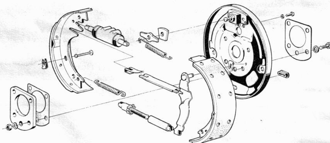
Bakhjulsbroms
