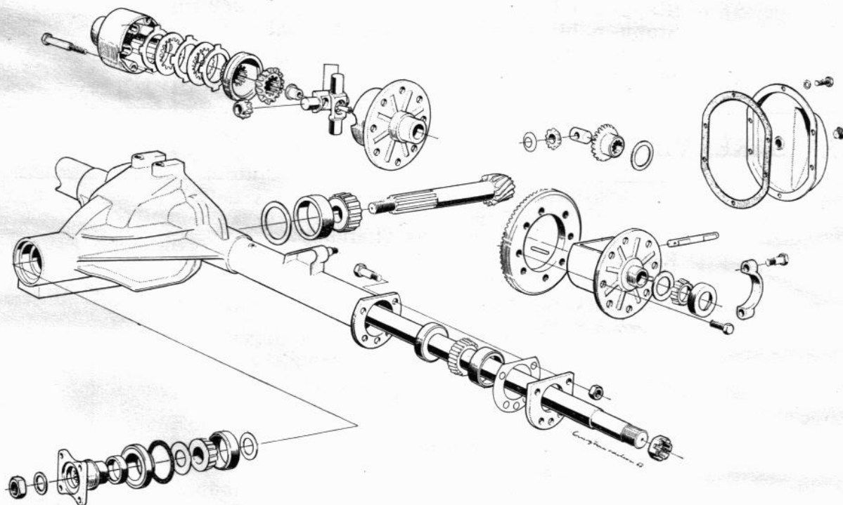
Bakaxel, fabrikat Spicer
